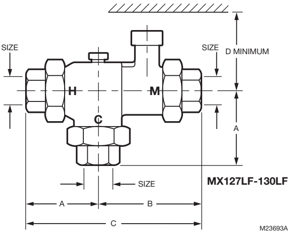
Fig. 1. Dimensions of Union NPT model.
