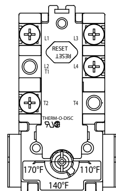
Figure 4. C-2 Thermostat
