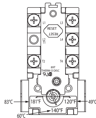
Figure 3. A-8 Thermostat
