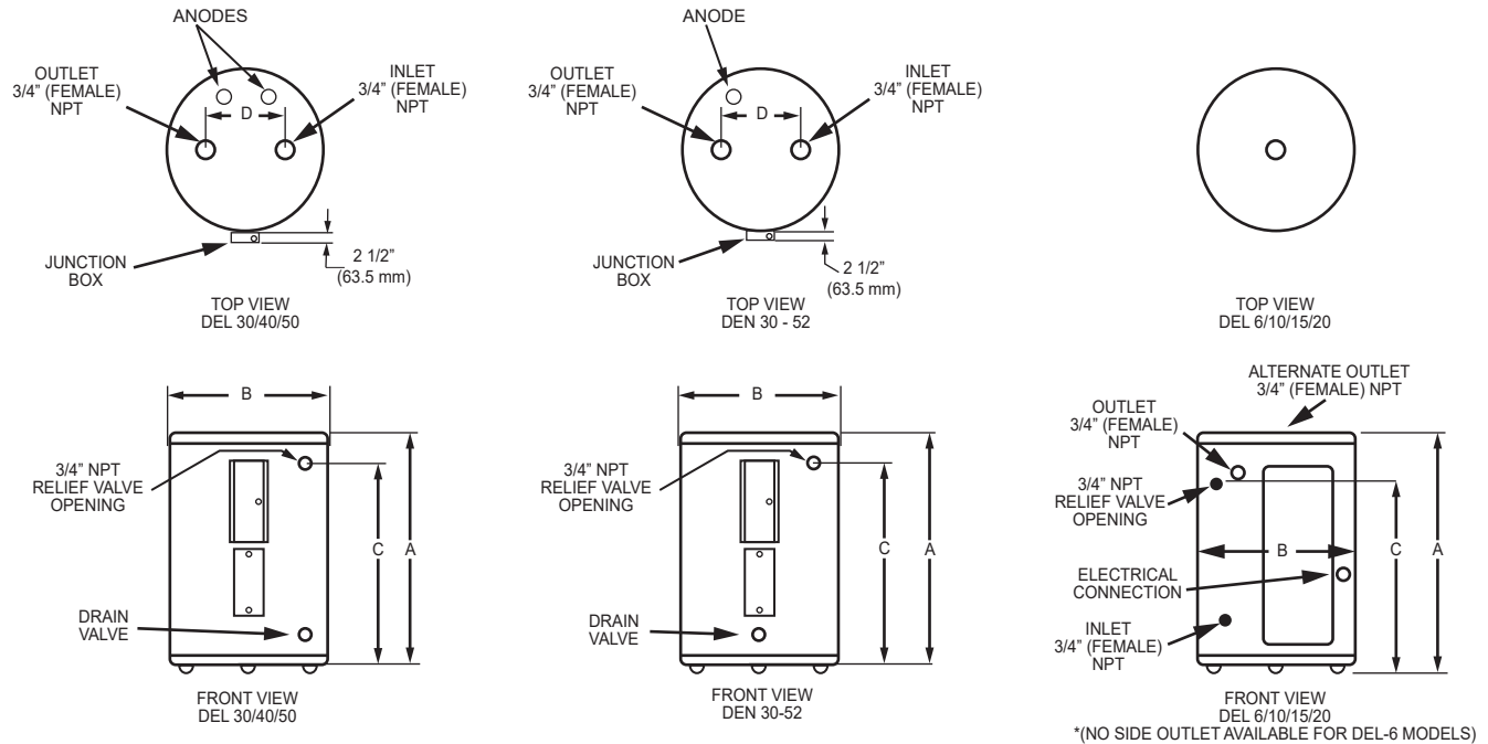
Figure 2. Rough-In Dimensions
