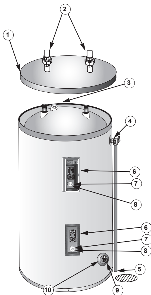
Figure 7. Leakage Checkpoints
