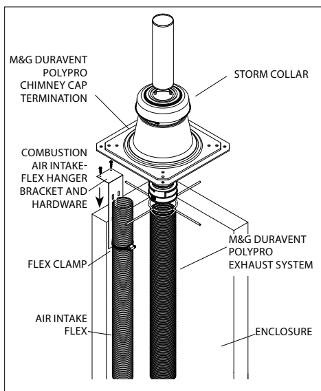
Figure 23- Upper Assy
