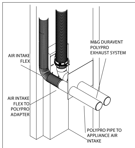
Figure 24- Lower Assy
