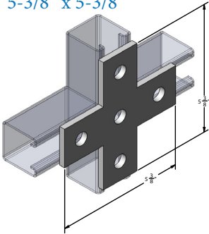
9017FF 4-hole cross plate 5-3/8" x 5-3/8"
