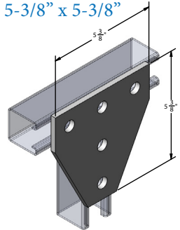
9019FF 5-hole tee gusset 5-3/8" x 5-3/8"
