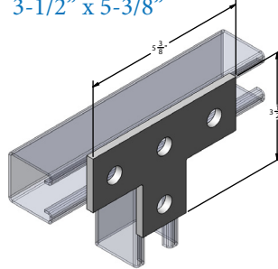
9016FF 4-hole tee plate 3-1/2" x 5-3/8"
