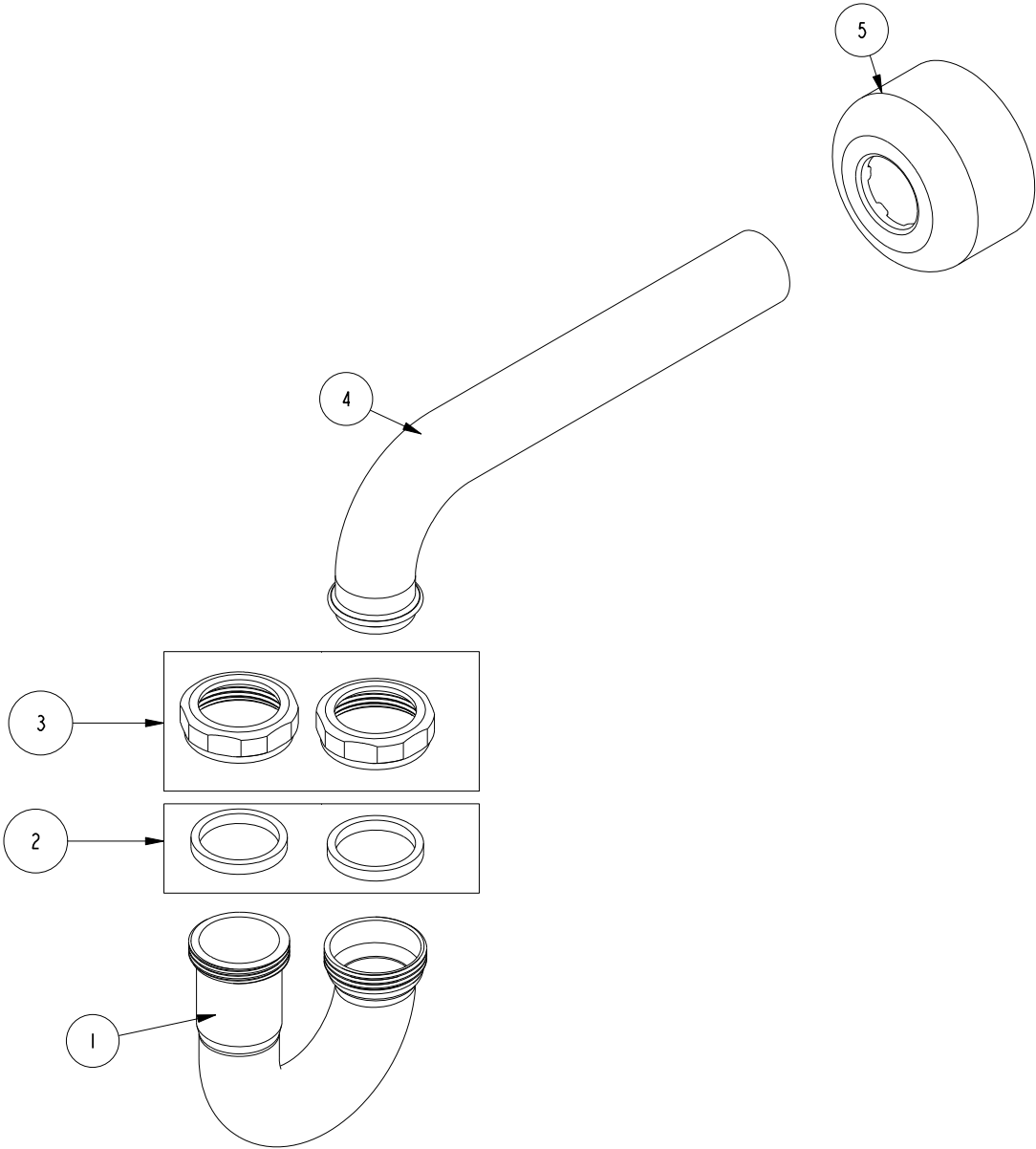
P-TRAP ASM 1-1/4" W/ BOX FLANGE 3014
