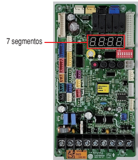
PCB principal
