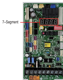
Main PCB
