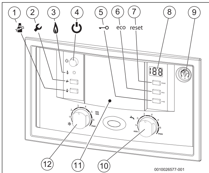
Fig. 2 Control panel
