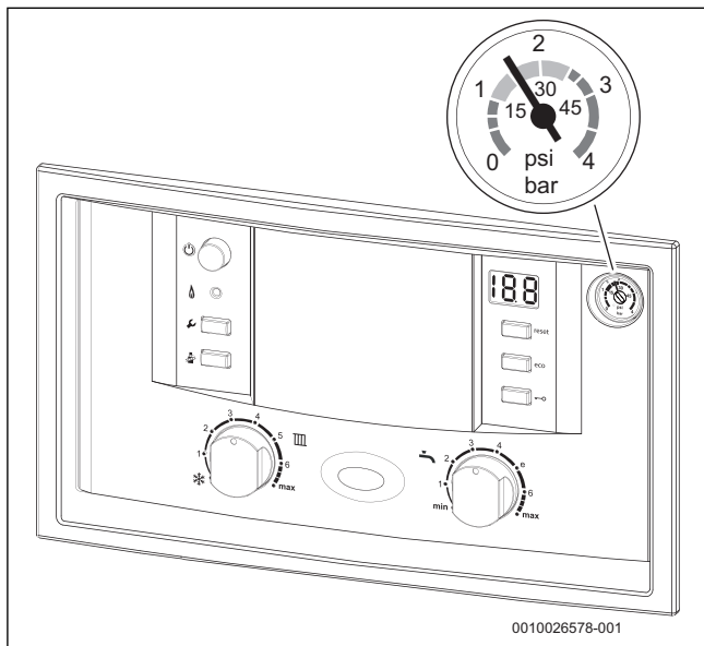
Fig. 1 Pressure gauge
