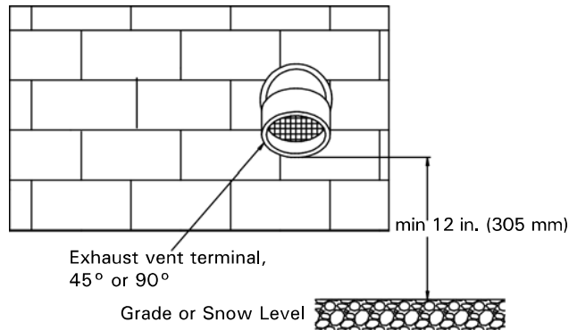
Side wall vent termination (front view)
