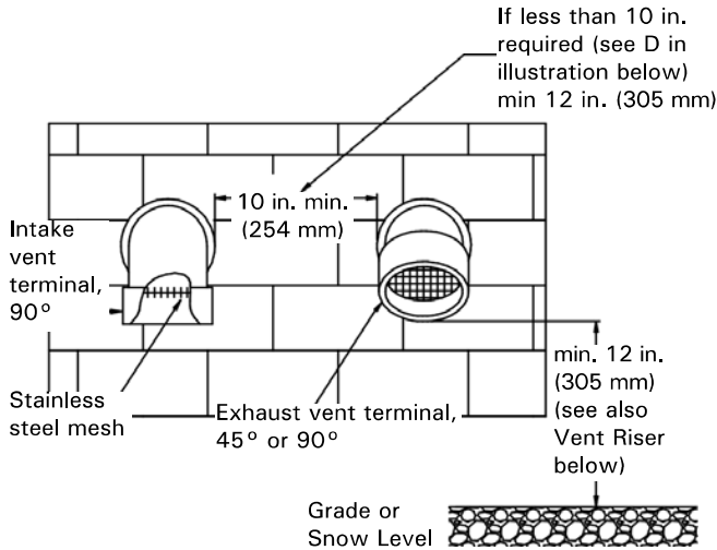
Side wall vent termination (front view)
