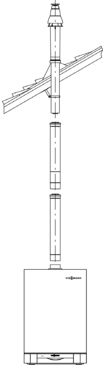
Sloped roof installation
