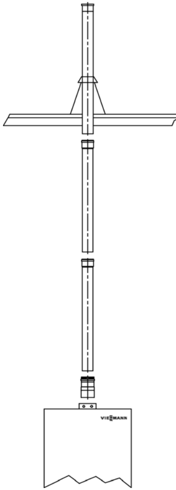
Flat roof installation
