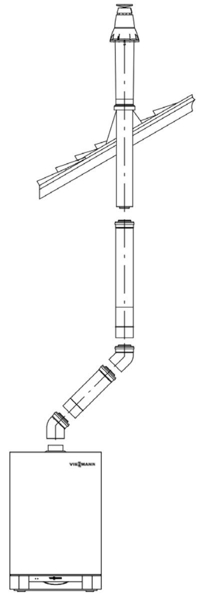
Sloped roof installation with offset
