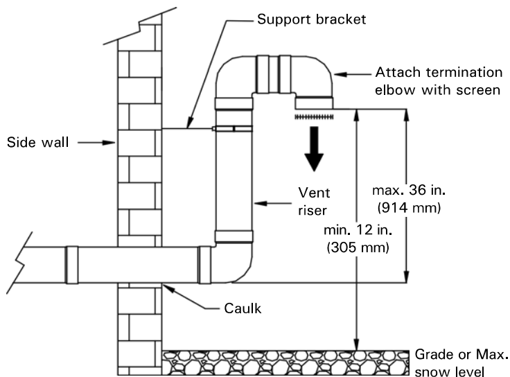
Installation of field supplied vent riser
