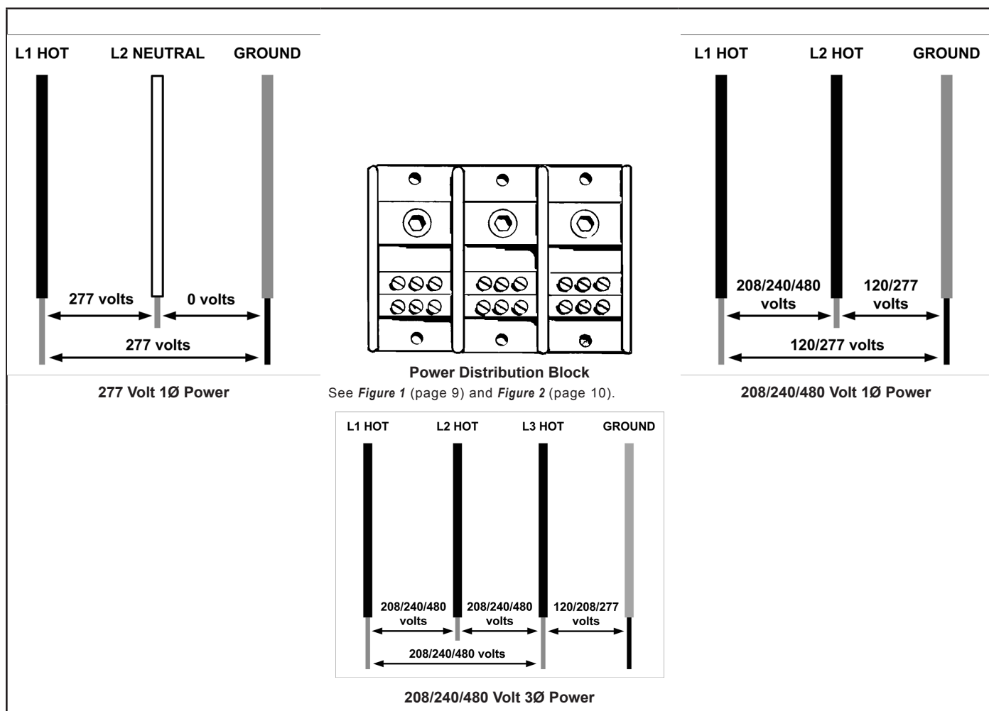
Figure 3. Wire Identification for Verification of Power Supply
