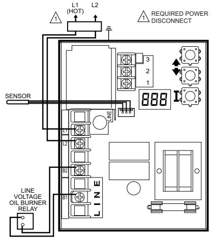
Fig. 5. L7103 connections.
