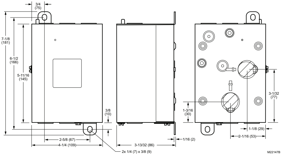
Fig. 1. L7103 mounting dimensions in in. (mm).
