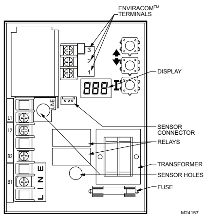
Fig. 3. Circuit board, showing sensor connection and well holes for vertical mount models.
