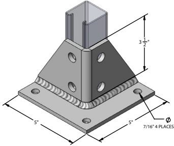
9090PB post base - flush mount for 1-5/8" x 1-5/8" strut.
