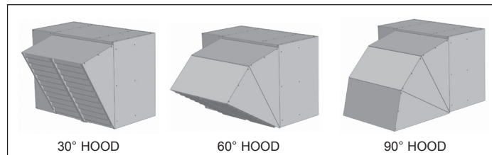
Figure 12.1 - 30°, 60°, & 90° Deflector Hoods
