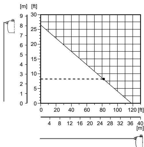
Maximum inlet-pipe length (horizontal axis) according to the suction lift (vertical axis)
